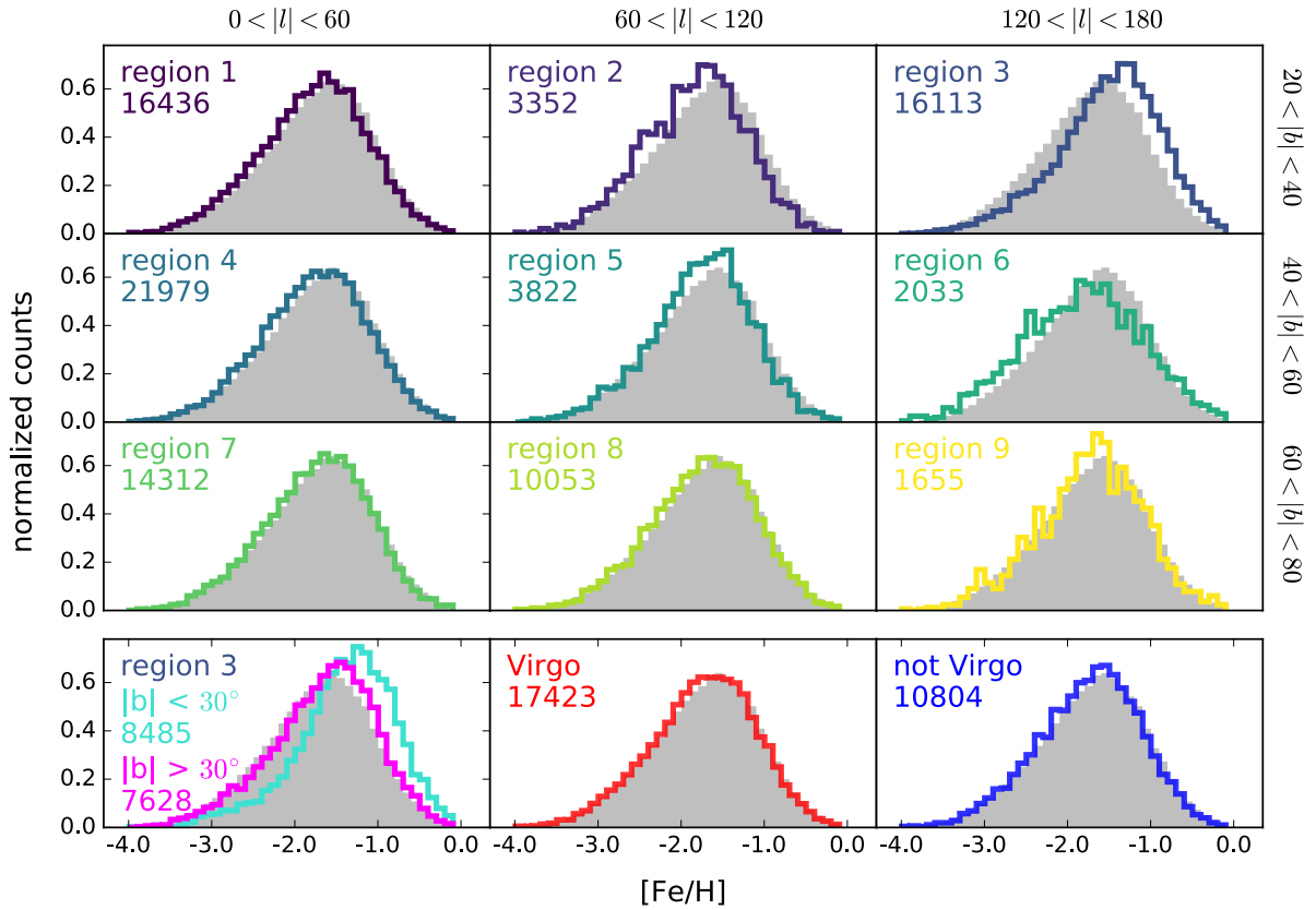
Figure 4.10 — MDFs for the 9 different regions described in the text, with colours that correspond to the numbered regions depicted in Figure 4.8. The grey filled histogram is the MDF of the total, GMM corrected halo sample for comparison. The bottom left panel shows the MDFs for region 3, separated into a high and low latitude sample (fuchsia and cyan, respectively), and the other two panels in the bottom row show the region selected to contain Virgo in red (the selected region is outlined in Figure 4.8), and the rest of the stars at the same Galactic latitude as a comparison are shown in blue.
