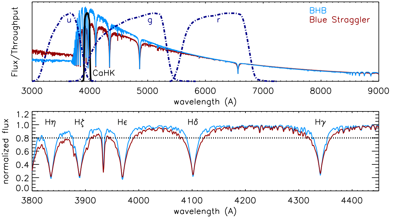
Figure 5.1 — Top panel: Synthetic spectra from a library of synthetic stellar spectra by Munari et al. (2005) for stars with stellar parameters T_{\text{eff}} = 8500 K and [\text{Fe}/\text{H}] = -0.5 . One of them has \log g = 3.0 (light blue, typical parameters for a BHB star) and the other one \log g = 5.0 (dark red, typical for a BS star) overplotted with the throughput curves for the SDSS ugr filters (dash-dotted dark blue lines) and the filter curve for the Pristine survey CaHK filter (thicker black line). Bottom panel: The same spectra, but now for a narrower wavelength range such that the Balmer series of hydrogen lines is plainly visible. The horizontal dotted line indicates a level of 0.8 in the normalized spectra where the widths of the hydrogen lines are traditionally measured to determine if the star is a BHB or BS star (see text for details).
