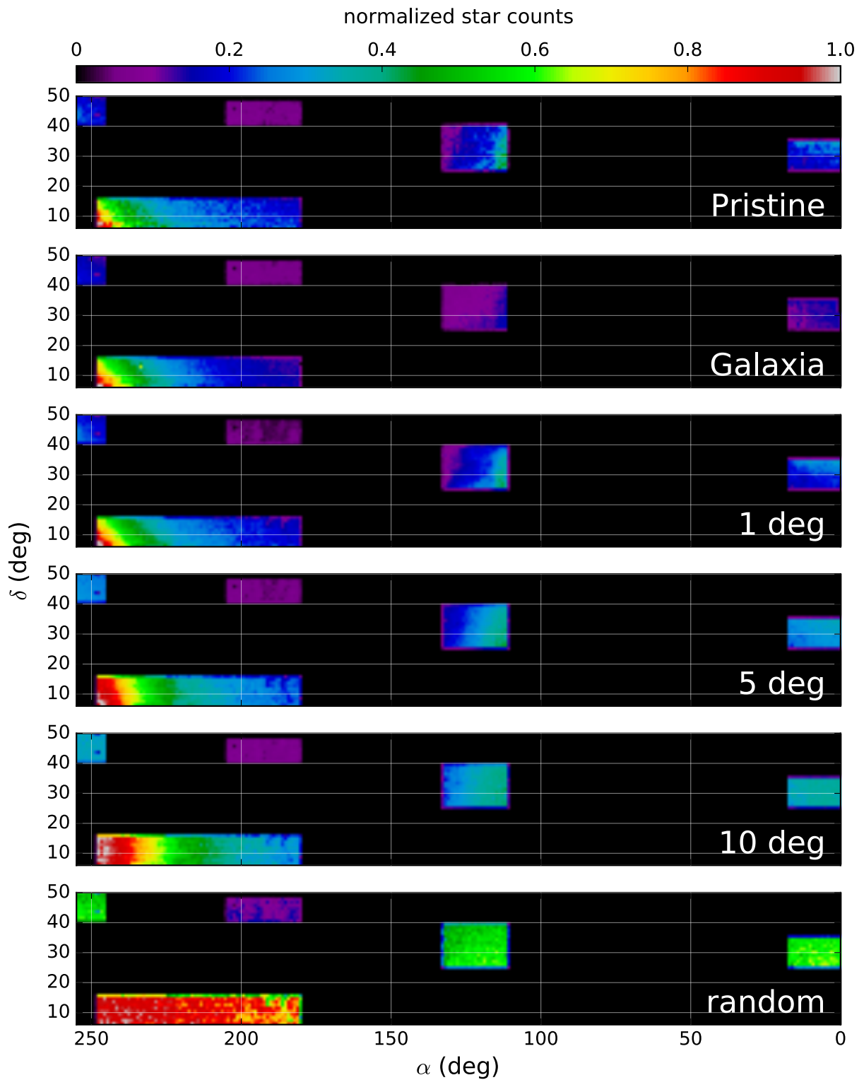
Figure 6.7 — Stellar density plots of the Pristine footprint (top) and the smooth background samples.
