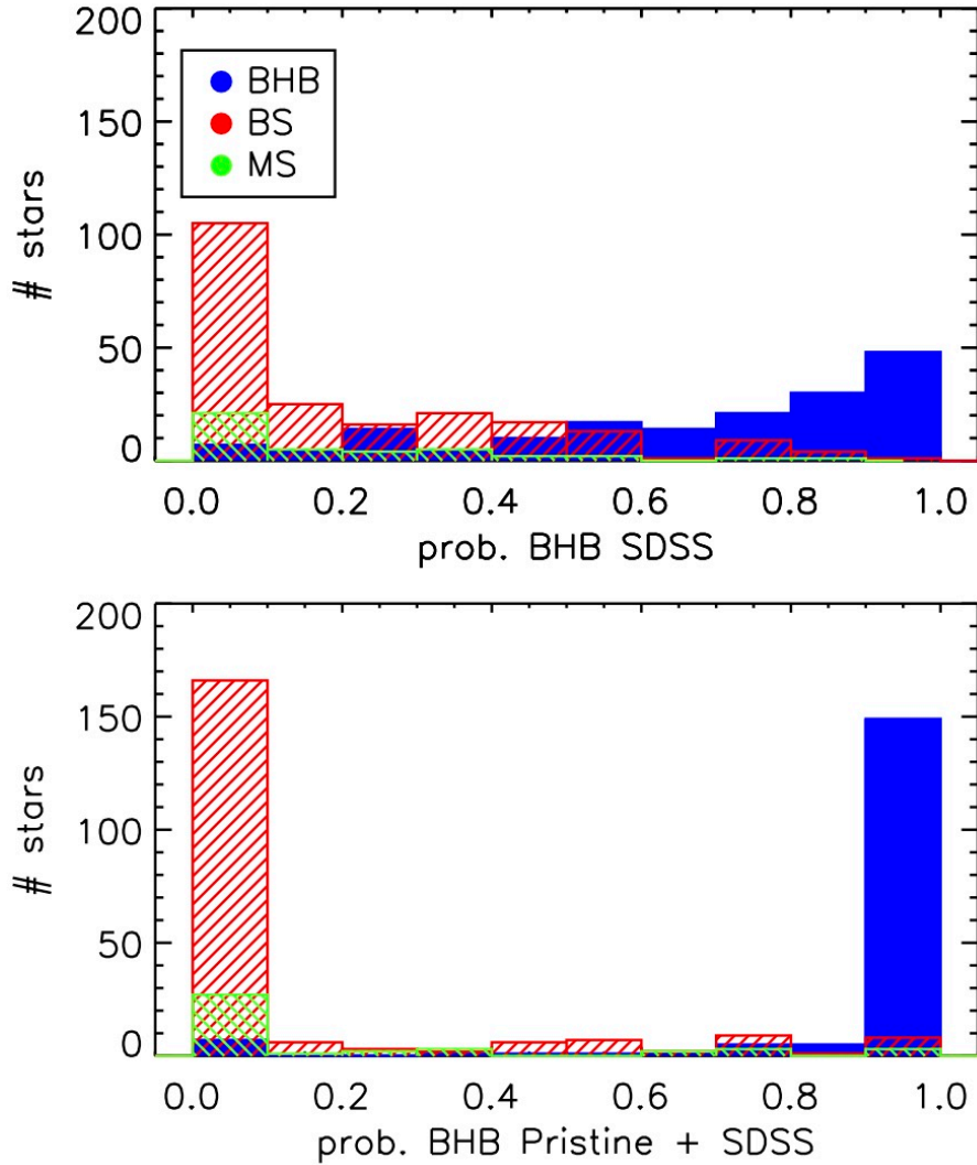
Figure 5.3 — The probability that stars from the Xue et al. (2008) spectroscopically followed up sample are BHB stars according to the methods presented in Sections 5.2.1 and 5.2.2 . The stars from Xue et al. (2008) are held against the same quality criteria (see text for details) and are separated in BHB (blue filled histogram), BS (red histogram), and MS (green histogram) stars according to the Xue et al. (2008) classification. It is clear that the addition of CaHK photometry adds to both the purity and completeness of a photometrically selected BHB sample.
