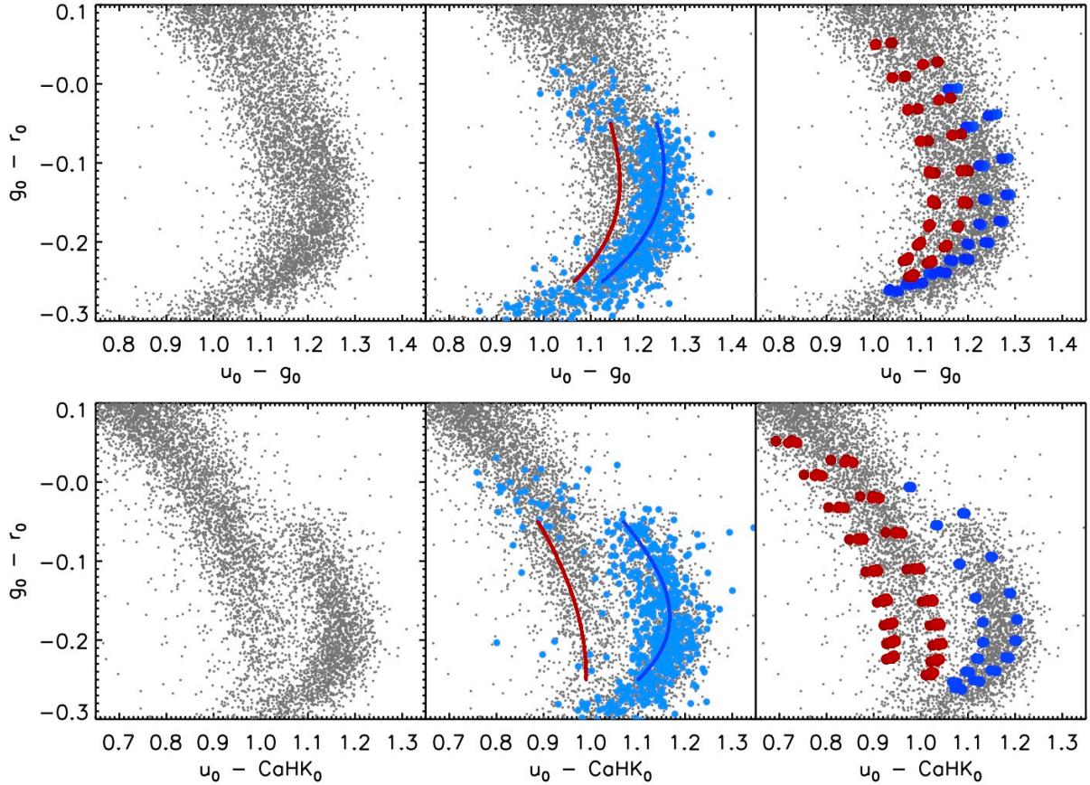
Figure 5.2 — Top panels: colour-colour space using SDSS broad-band data for a selected sample of clean photometry for hot stars (see text for details). In the middle, the ridgelines defined in Deason et al. (2011) for BHB and BS stars (blue and red lines respectively) are plotted on top of the BHB sample of Xue et al. (2011) (light blue filled circles). In the right panel, the results from synthetic colours for spectra from the Munari et al. (2005) library with typical BHB (blue points; -2.5 < [\text{Fe}/\text{H}] < -1.5 , 7\,500 < T_{\text{eff}} < 9\,500 K, 3.0 < \log g < 3.5 ) and BS (red points; -1.0 < [\text{Fe}/\text{H}] < -0.5 , 7\,500 < T_{\text{eff}} < 9\,500 K, 4.0 < \log g < 4.5 ) stellar parameters are overplotted. Bottom panels: The same stellar sample as in the top panels, but now for a colour-colour space combining the SDSS and the Pristine survey photometry. The ridgelines are defined in this work and described in the text.
