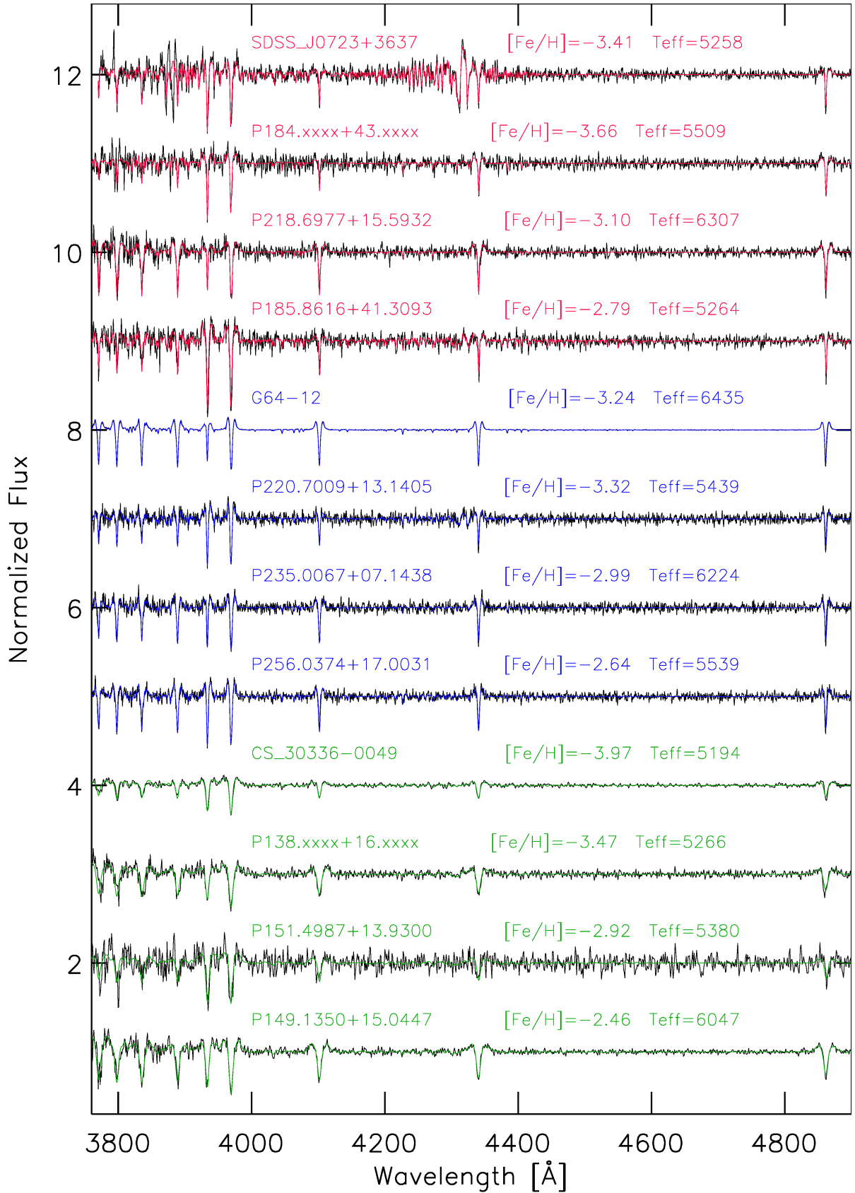
Figure 3.3 — A subsample of the spectra of the Pristine candidates observed with IDS/INT (red), ISIS/WHT (blue), and EFOC/3.6 NNT (Green) together with the best fit derived with FERRE. Three well known metal-poor stars are shown for comparison, SDSS J0723+3637, G64-12, and CS 30336-0049. The main stellar parameters are also displayed.
