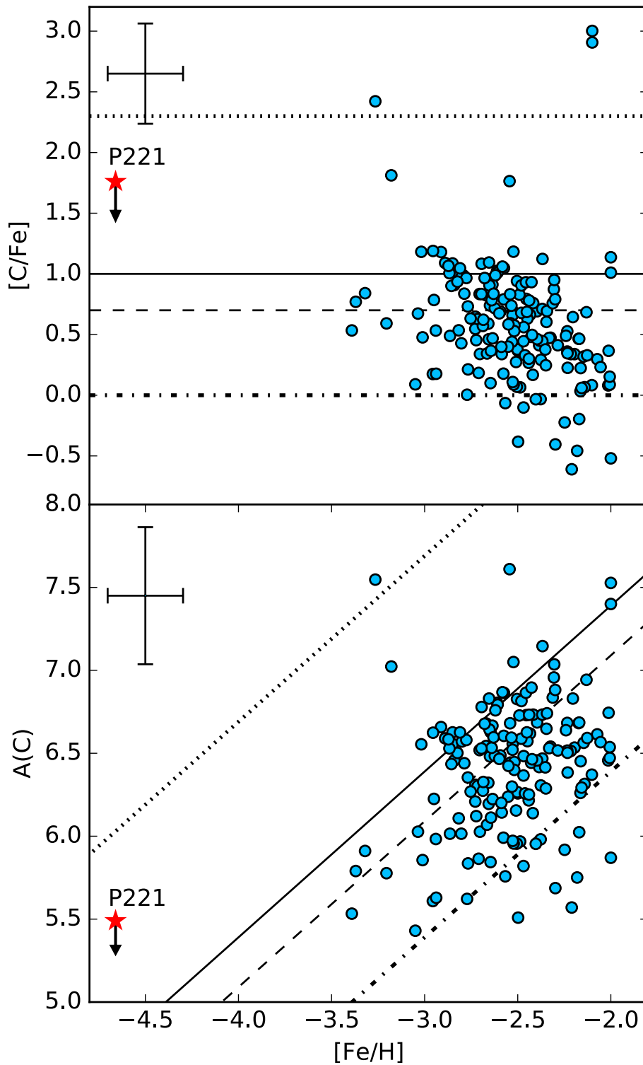
Figure 3.8 — Carbon vs iron for [\text{C}/\text{Fe}] (top) and absolute carbon (bottom). The red star represents Pristine _221.8781+9.7844, with parameters derived from the analysis of a high-resolution UVES spectrum (Starkenburger et al. 2018). The dashed-dotted line at [\text{C}/\text{Fe}] = 0 shows the solar carbon abundance, the dashed and solid lines at [\text{C}/\text{Fe}] = +0.7 and +1.0 show the thresholds for carbon enhancement defined in Aoki et al. (2007) and Beers et al. (2005), respectively, and the dotted line at [\text{C}/\text{Fe}] = 2.3 shows the boundary of the silicate dominated region, as described in Chiaki et al. (2017). The error bars shown in the top left of each panel represent the median errors of the sample.
