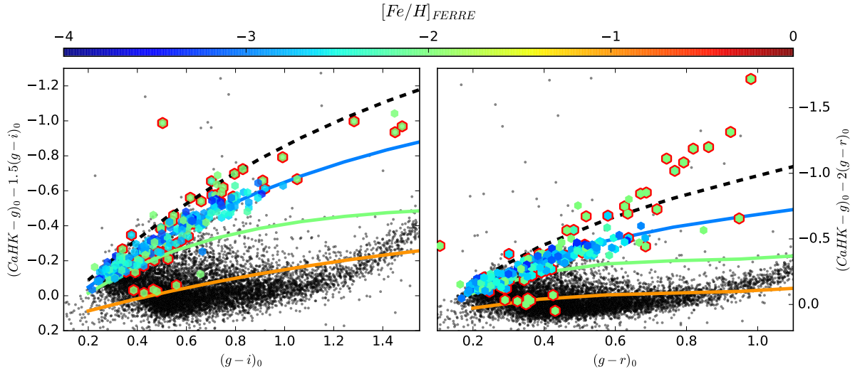
Figure 2.5 — The same colour-colour space as in Figure 2.1 but with stars that have been selected for spectroscopic follow-up coloured according to their spectroscopic [\text{Fe}/\text{H}]_{\text{FERRE}} . The coloured lines trace along constant metallicities and the black dashed line is the expected limit of stars that have no metal absorption lines in their spectra. The grey points are 10 000 randomly selected Pristine stars, to show the parameter space covered by the survey. Data points circled in red represent the stars that are removed from the sample by the selection criteria, many of which are contaminants with [\text{Fe}/\text{H}]_{\text{FERRE}} \geq -2 . These stars circled in red are listed at the bottom of Table 2.1
