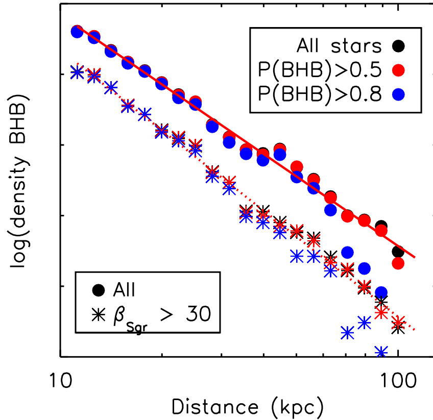
Figure 5.9 — Distance profile (in arbitrary units) of BHB stars selected in three different ways: either by taking all stars with a probability that they are a BHB star higher than 0.5 (red filled circles), or 0.8 (blue filled circles), or by taking all stars that pass the quality cuts and multiplying them with the probability they represent BHB stars (black filled circles). A fit to the red symbols is illustrated and has a negative power-law slope of 3.5 \pm 0.1 (for the full sample), or 4.0 \pm 0.1 for the sample at least 30 degrees off the Sagittarius orbital plane. These profile fits are shown by the full and dotted red lines respectively.
