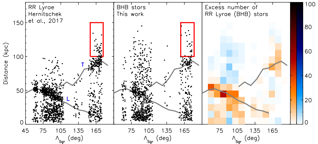
Figure 5.11 — RR Lyrae (left panel, taken from Hernitschek et al. (2017) ) and BHB stars (second panel, this work, selected to have P(\text{BHB} | u\text{CaHKgr}) > 0.5 ) as a function of longitude along the Sagittarius orbital plane and heliocentric distance. Grey lines guide the eye along Sagittarius stream components as defined by the RR Lyrae measured by Hernitschek et al. (2017) . Blue letters ‘L’ and ‘T’ indicate the leading and trailing arm respectively. Red boxes illustrate the distant “spur” feature discovered in the same RR Lyrae sample ( Sesar et al. 2017a ). The third panel illustrates the difference in both populations by either counting the excess of RR Lyrae stars (red colour bar), or BHB stars (blue colour bar).
