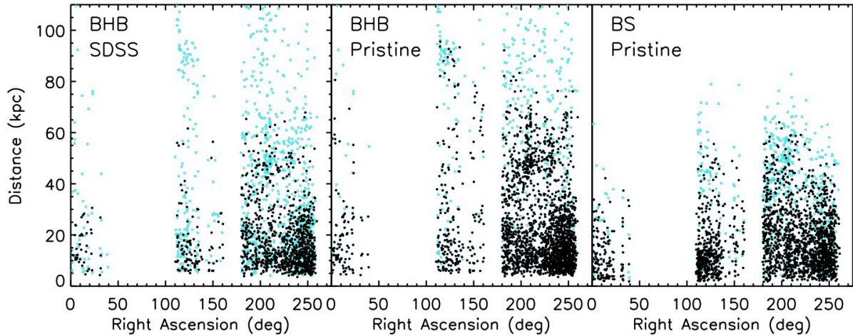
Figure 5.7 — Right ascension versus distance maps for the three different populations shown in Figure 5.6. Stars with a probability > 0.8 per class are shown in black, while stars with a probability between 0.5 and 0.8 appear as cyan points.
