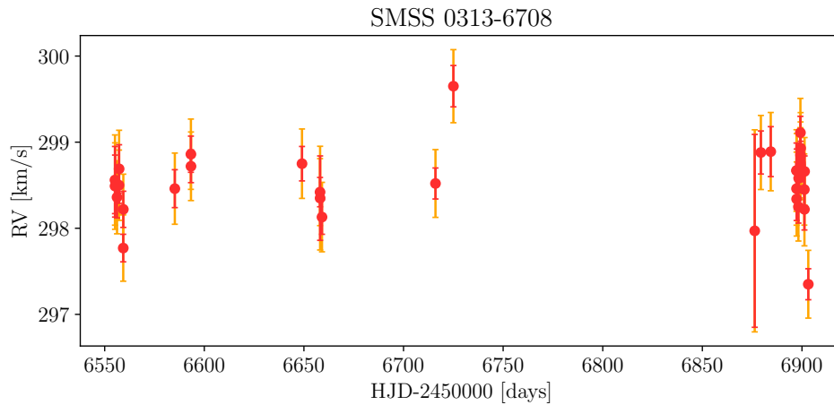
Figure 2.12 — Radial velocities for SMSS 0313–6708, derived from archive UVES spectra. The red error bars represent the uncertainties coming from EXCOR, and the orange error bars include an uncertainty floor of 0.35 \text{ km s}^{-1} .
