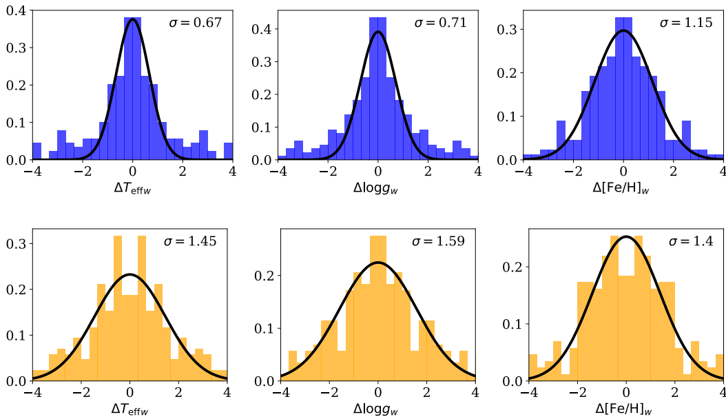
Figure 3.3 —Distributions of \Delta P_w for pairs of observations of the same star. The UVB and VIS analyses are presented in the top and bottom row, respectively. The Gaussians with a mean of zero and a standard deviation computed as described in the text are shown, the standard deviations of these Gaussians are given in the top right corner of each panel.
