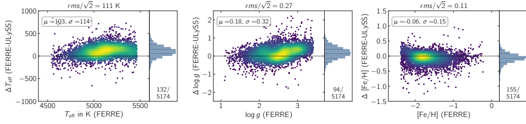
Figure 5.6 — Comparison of the parameters between ULYSS and FERRE colour-coded by density, for giant stars ( \log g < 3.5 ) cooler than 5500 K and with [\text{Fe}/\text{H}] > -2.5 . The zero-line is indicated. The mean difference and standard deviation are indicated in the top left corner of each main panel, after discarding 3\sigma outliers. The number of outliers versus the total number of stars are indicated on the bottom of the histogram panels. Finally, the title of each panel includes the corresponding rms/\sqrt{2} , which is quadratically added to the internal uncertainties from Section 5.3.4 and 5.3.5 to derive total uncertainties for both analyses.
