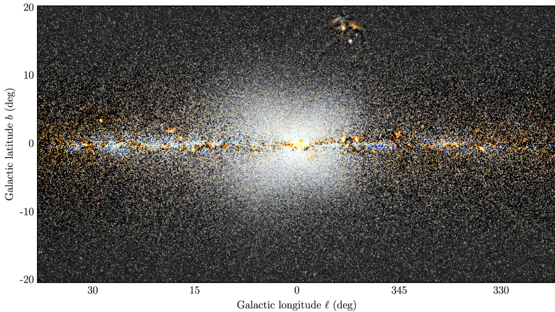
Figure 1.4 — WISE photometry from the W1 and W2 bands in Galactic coordinates towards the bulge. In this image, the median of each row of the image has been subtracted for contrast. Image from Ness & Lang (2016) .
