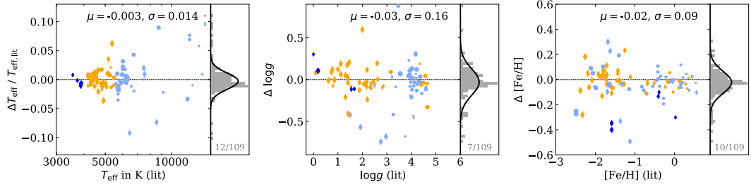
Figure 3.10 — Comparison between our adopted parameters and the parameters from Wu et al. (2011a) . One and three outliers are not shown for \log g and [\text{Fe}/\text{H}] , respectively, and one measurement at 29000 K is not shown (its \Delta T_{\text{eff}} / T_{\text{eff, lit}} is +0.027.). The axes and symbols are explained in Figure 3.8
