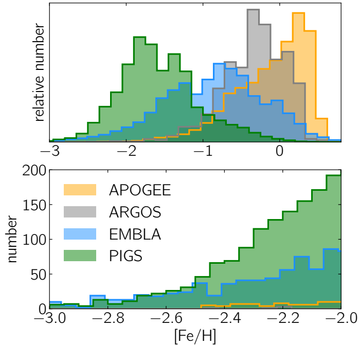
Figure 5.8 — Top panel: Relative metallicity distribution of PIGS ([Fe/H] from FERRE), EMBLA, three fields of the ARGOS survey at (l, b) = (5^\circ, -5^\circ) , (5^\circ, -10^\circ) and (10^\circ, -10^\circ) , and all stars from APOGEE DR16 (using [M/H]) in the region |l|, |b| < 12^\circ . Bottom panel: absolute number of VMP stars in the same samples.
