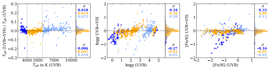
Figure 3.6 — Difference between the parameters determined from the UVB and VIS spectra for stars with 3500 \text{ K} < T_{\text{eff}}(\text{UVB}) < 10000 K. The colour-coding is the same as in Figure 3.5, and for the coolest stars ( < 4000 K) the giants are shown with crosses. In the \log g panel, two outliers (hot stars) are not shown. The dispersion \sigma and mean offset \mu for the three temperature ranges are indicated.
