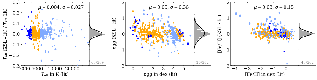
Figure 3.8 — Comparison between our adopted parameters and the literature compilation. The standard deviation and mean of the differences are written and the corresponding curve is shown. The number of clipped observations compared to the total number of literature values is presented in the lower right corner of each of the panels. The colour of the points relates to T_{\text{eff}} ; the size of the points to [\text{Fe}/\text{H}] , and giants and dwarfs ( \log g limit 3.0) are indicated by diamonds and circles, respectively. In the T_{\text{eff}} and \log g panels, two and four outliers, respectively, are not shown (various types of stars).
