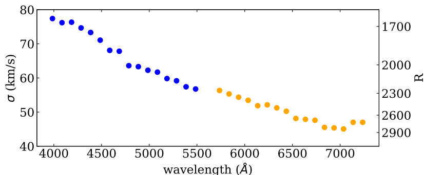
Figure 3.2 — Line spread function for the MILES interpolator, separated by colour for the UVB and VIS.
