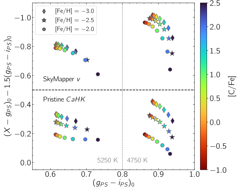
Figure 6.3 — Synthetic photometry from model spectra with the SkyMapper (top) and Pristine (bottom) filters, for the same T_{\text{eff}} and \log g as the models in Figure 6.2 (5250 K on the left, and 4750 K on the right). The results for SkyMapper have been offset by 0.3 mag to separate the SkyMapper and Pristine results.
