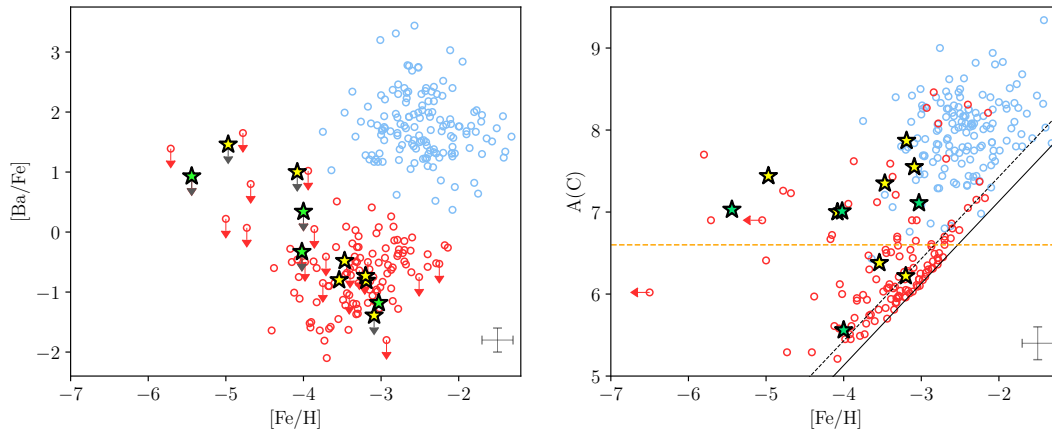
Figure 2.7 — Left: [\text{Ba}/\text{Fe}] as a function of [\text{Fe}/\text{H}] for the compilation of CEMP stars from Yoon et al. (2016) down to [\text{Fe}/\text{H}] = -6 , where CEMP- s stars are shown in blue and the CEMP-no stars in red. The known and new CEMP-no binaries are indicated as yellow and green stars, respectively. Right: The same, but for A(\text{C}) on the y-axis. The solid and dotted black lines indicate the [\text{C}/\text{Fe}] > +0.7 and [\text{C}/\text{Fe}] > +1.0 CEMP criteria, respectively. The orange dashed line indicates the separation of the low- and the intermediate-/high-carbon band. For both panels, typical error bars on the abundances are shown in the lower right corner.
