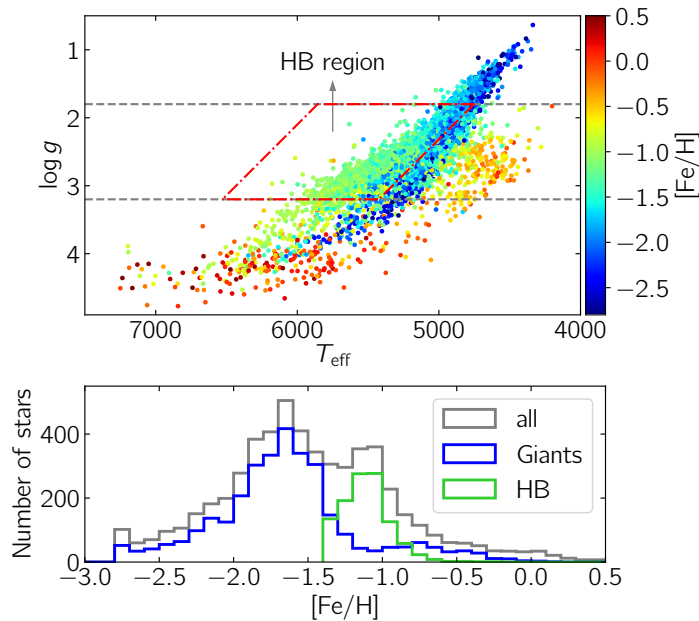
Figure 4.2 — Top: T_{\text{eff}} – \log g diagram colour-coded by [\text{Fe}/\text{H}] , for the sample making our quality cuts. The the \log g cuts are indicated in grey, and the box containing HB stars is shown in red (see Section 4.5.2 in the Appendix). Bottom: Metallicity distribution of our full sample in grey, with the 4200 stars that have 1.8 < \log g < 3.2 highlighted in blue (giants) and green (HB stars). The lower [\text{Fe}/\text{H}] limit of the interpolator is -2.8 , causing an apparent excess of stars there.
