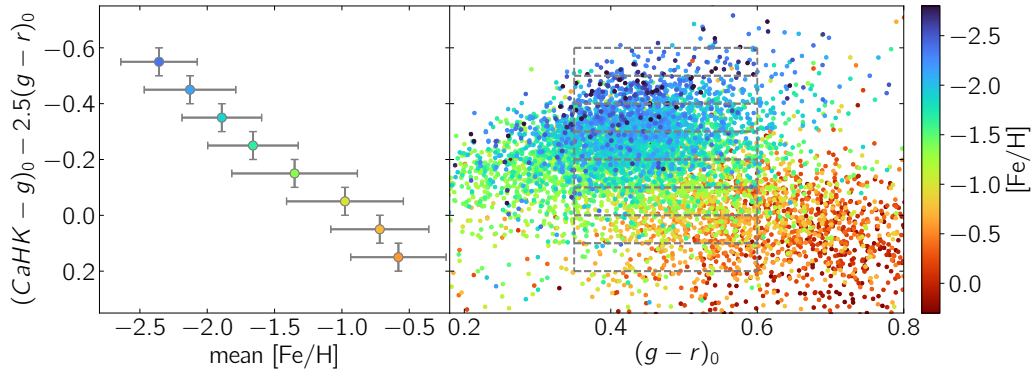
Figure 5.9 — Mean metallicity in bins of the y-axis of the Pristine colour-colour diagram (left) and the corresponding diagram with the indicated bins (right). Error bars in the left panel are the 1\sigma dispersion in each bin for [Fe/H] , and for the y-axis they indicate the size of the bin. Included are stars from PIGS (using their FERRE [Fe/H] ), and stars from EMBLA, APOGEE DR16 (using [M/H] ) and ARGOS. Only stars with E(B-V) < 0.6 are included.
