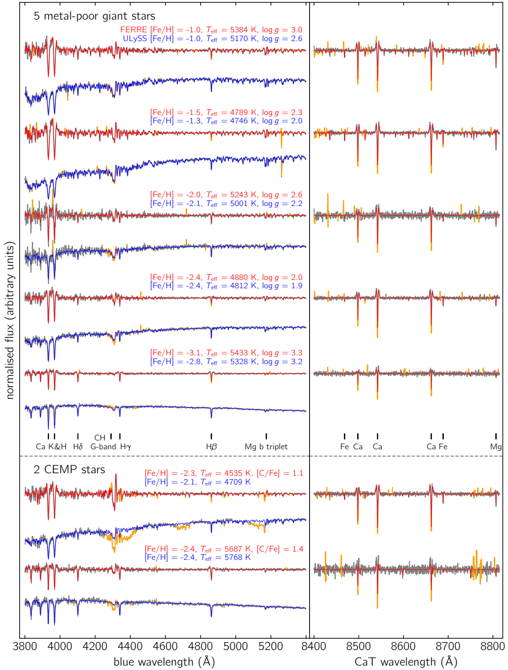
Figure 5.4 — Example fits for ULYSS (blue) and FERRE (red) for five metal-poor giants and two CEMP stars. For both analyses, the observed (normalised) spectrum is shown in grey. Regions in the observed spectra which are masked in the fit are indicated in orange, these contain both a priori masks (the CH G-band in ULYSS and the calcium triplet line cores in FERRE) and pixels that are masked iteratively. Several of the strongest spectral features have been indicated. For each star, the stellar parameters from both analyses are given. The \text{SNR}_{4000-4100} varies between 12 – 47, and \text{SNR}_{\text{CaT}} between 28 – 96.
