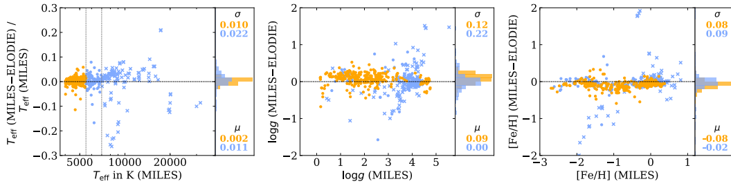
Figure 3.4 — Comparison between the MILES and ELODIE solutions in the UVB for the stars with T_{\text{eff}}(\text{MILES}) > 4000 K. Each atmospheric parameter is shown in a separate panel, and the colour of the symbols identify two temperature ranges (dividing at 5500 K). Stars hotter than 7000 K are shown as crosses. In the T_{\text{eff}} and \log g panels, seven and two outliers, respectively, are not shown (all hot stars). The dispersion \sigma and mean offset \mu for the two temperature ranges are indicated.
