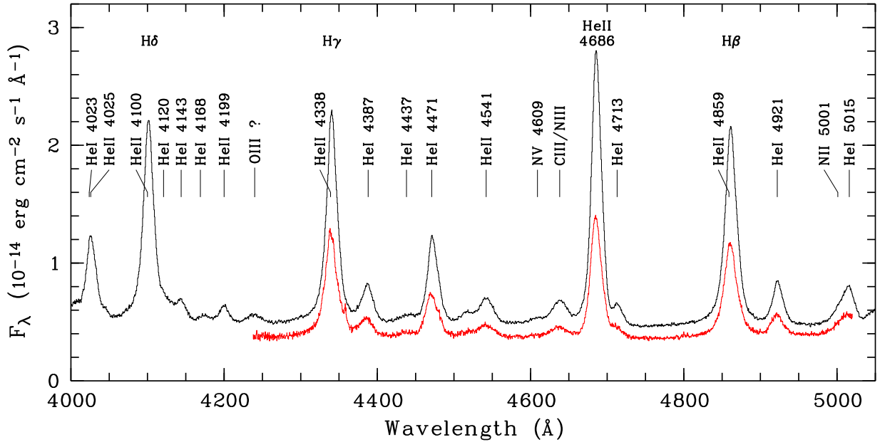
Fig. 1. Flux-calibrated average spectra of BY Cam obtained on November 19, 1998 (bottom) and December, 19 1999 (top).
