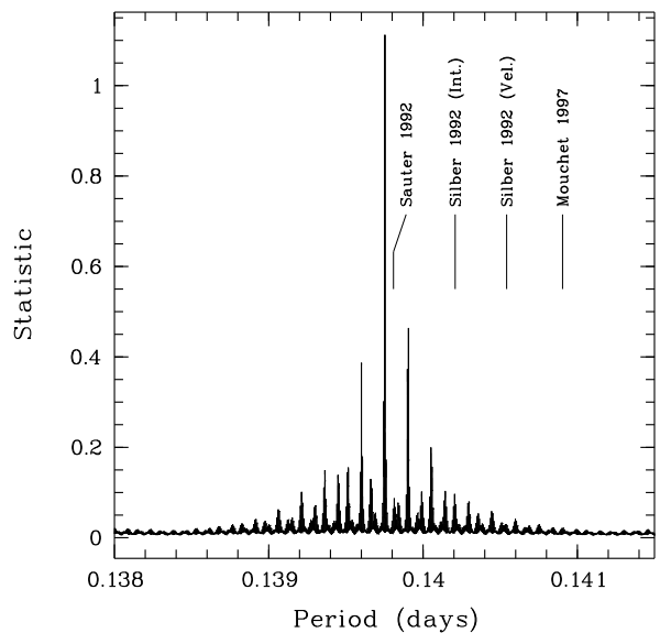
Fig. 4. Periodogram using the \chi^2 method applied to the timings of blue-red zero-crossings of the narrow component of the Balmer lines. The likely period of 0.139791 days (201.199 min) and other spectroscopic measurements of the orbital period are indicated.
