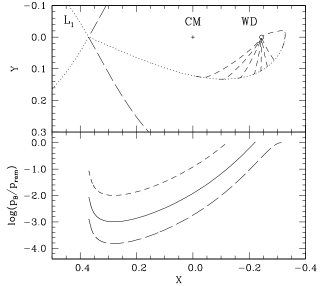
Fig. 5. upper panel) Geometry of the suspected accretion curtain projected onto the orbital plane. Assumed are system parameters and a dipole orientation as outlined in Sect. 3.2. Indicated are the Roche lobes of both stars, the L_1 -point, the white dwarf and the centre of mass. The curtain is represented by 8 magnetic trajectories, also shown in velocity coordinates (Fig. 3). coupling occurs over a range of azimuth from \psi_{\text{thread}} = 35^\circ to 175^\circ . lower panel) The ratio of magnetic and ram pressure along the stream, for three exemplary mass accretion rates ( \dot{M} = 1 \times 10^{-11}, 1 \times 10^{-10}, 6.6 \times 10^{-10} M_\odot \text{ yr}^{-1} ) needed to reach the range of coupling radii implied by the extent of the accretion curtain.
