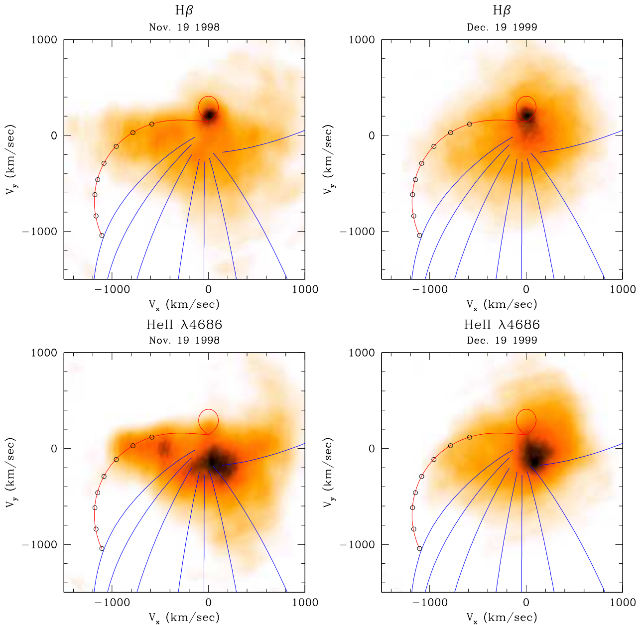
Fig. 3. Doppler maps of BY Cam computed from H\beta and He\ II\ \lambda 4686 emission lines observed in 1998 and 1999. Overlaid are the locations of the secondary star, a ballistic trajectory (both red), and a set of magnetic trajectories representing an extended curtain (blue). Small circles mark the positions where those trajectories are leaving the ballistic stream.
